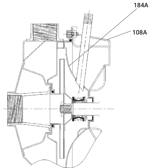
Seal face vent/flush option
