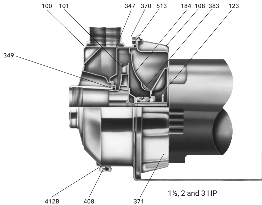
Seal face vent/flush option
